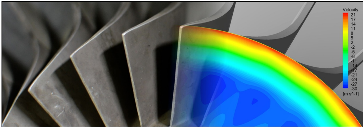
Centrifugal compressor flow velocity map calculated on ARCHIE-WeSt. Image provided by Grzegorz Liśkiewicz, University of Strathclyde / Lodz University of Technology
