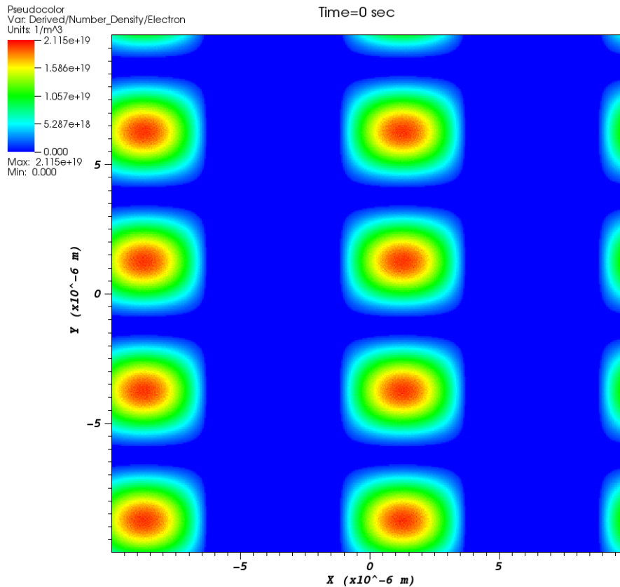
Figure 8: Complex 2D density structure
